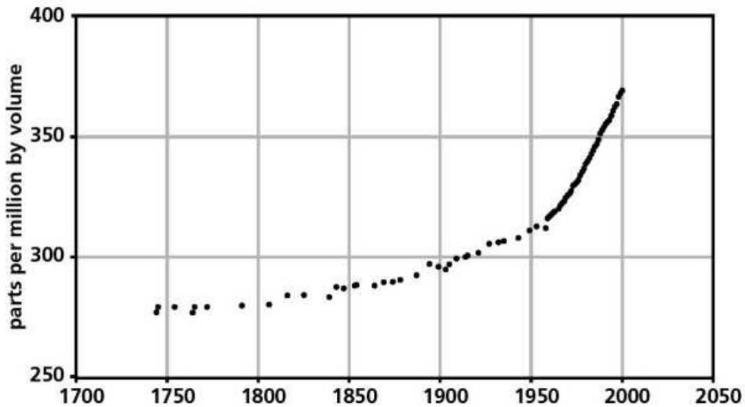
FIGURE 1-3 Carbon Dioxide Concentration in the Atmosphere
