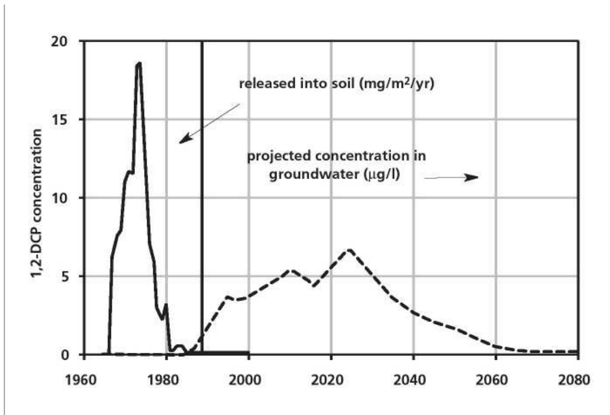
FIGURE 4-10 The Slow Percolation of 1,2-DCP into Groundwater
