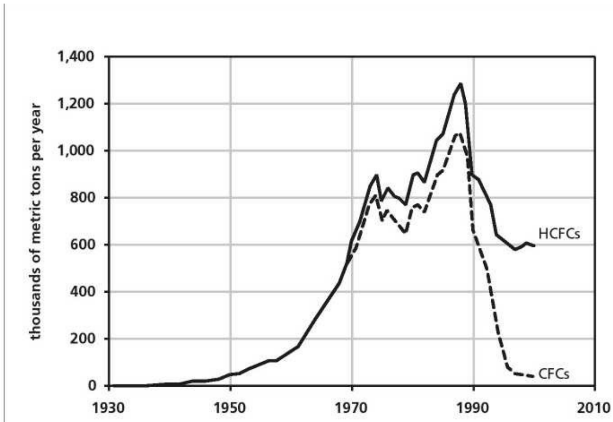
FIGURE 5-1 World Production of Chlorofluorocarbons
