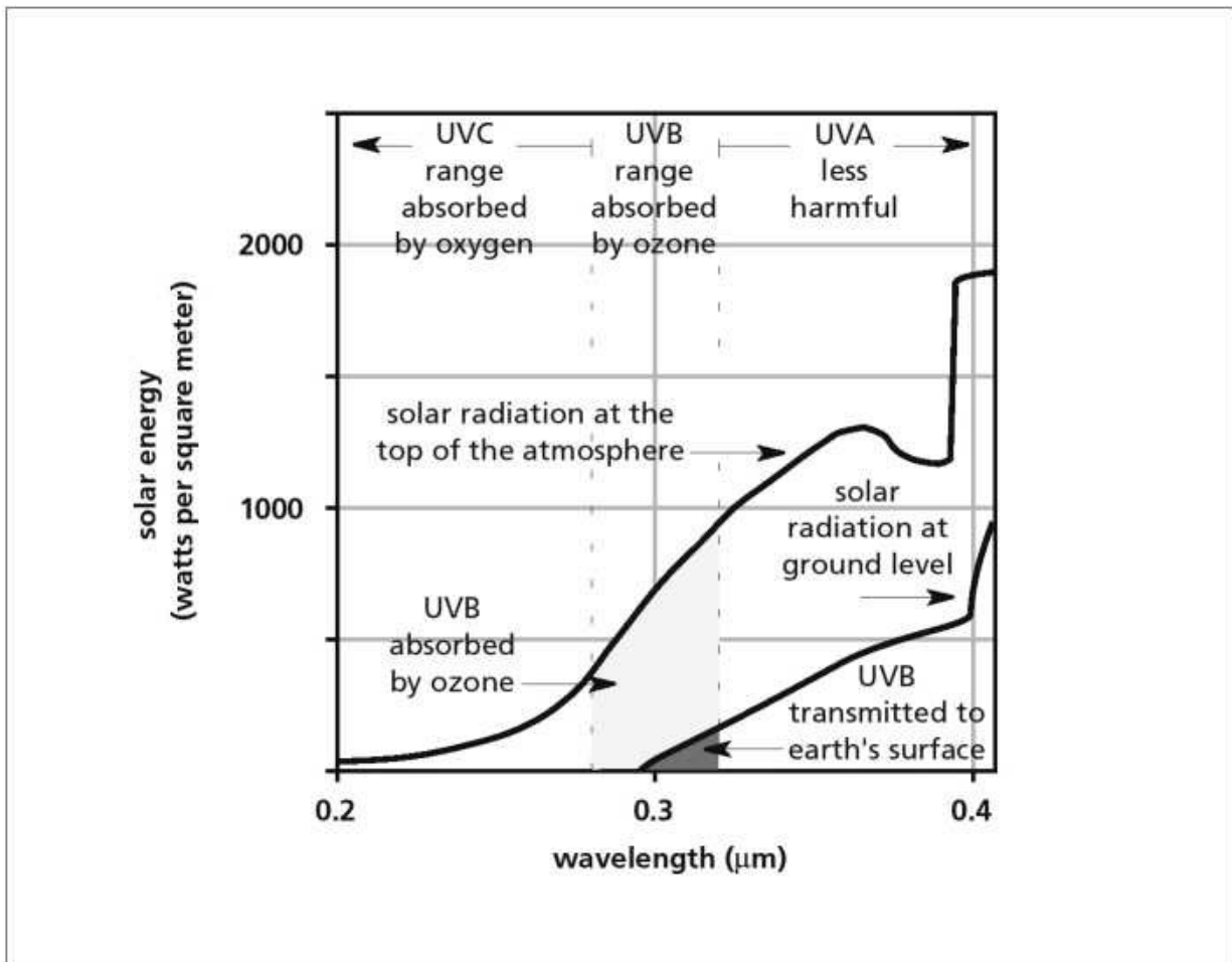
FIGURE 5-2 Absorption of Light by the Atmosphere
