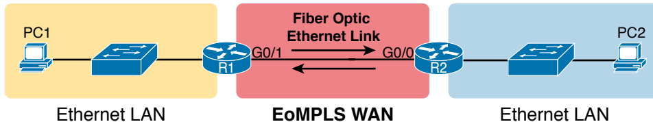
Figure 3-8 EoMPLS Acting Like a Simple Ethernet Link Between Two Routers
