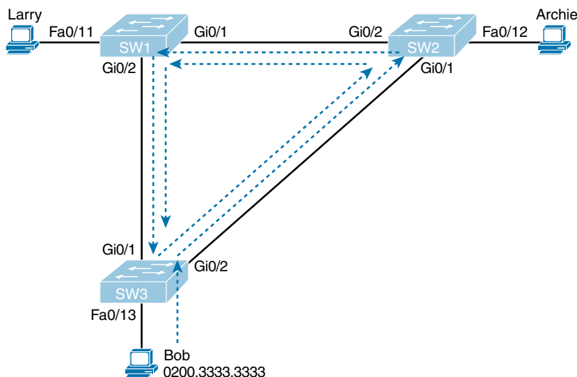
Figure 9-1 Broadcast Storm
