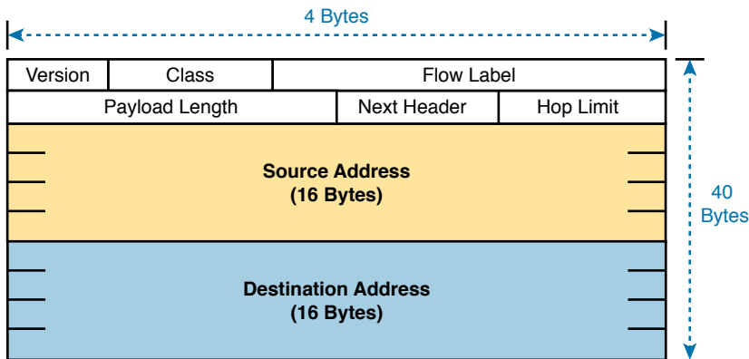
Figure 22-3 IPv6 Header
