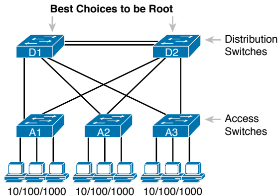
Figure O-1 Typical Configuration Choice: Making Distribution Switch Be Root
