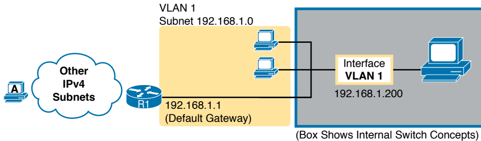
Figure 6-8 The Need for a Default Gateway
