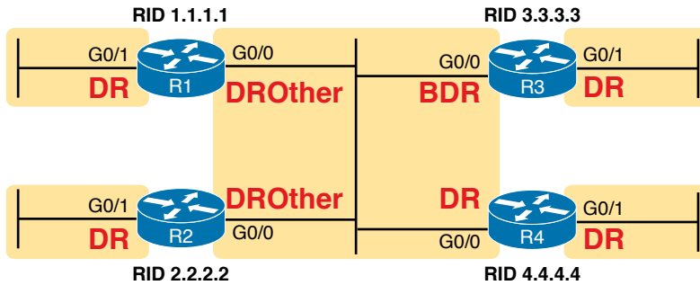
Figure 21-2 OSPF DR/BDR/DROther Roles in the Network
