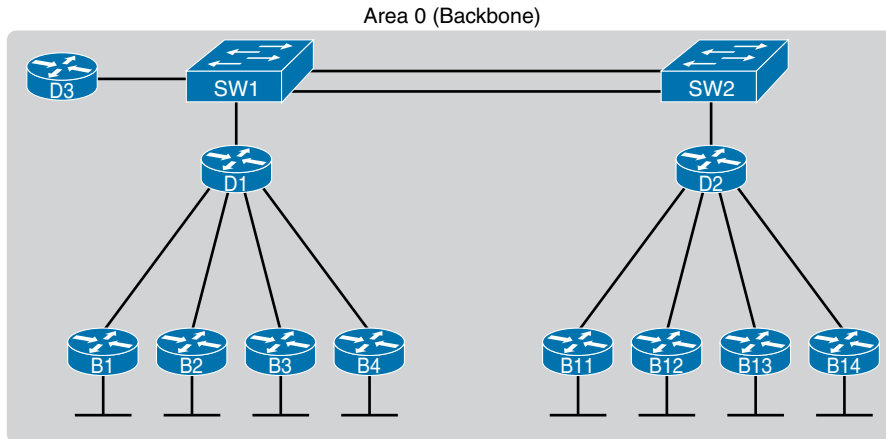
Figure 19-12 Single-Area OSPF
