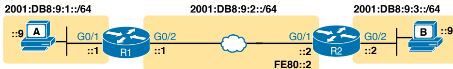
Figure 25-7 Sample Topology for Incorrect IPv6 Route Examples
