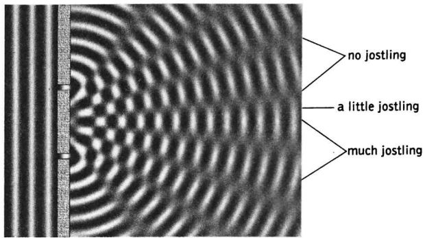
Figure 4.7 Circular water waves that emerge from each slit overlap with each other, causing the total wave to be increased at some locations and decreased at others.
