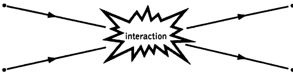
Figure 6.5 Two particles interact—they “slam together”—and cause the path of each to be deflected.
