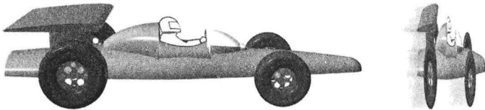
Figure 2.4 A moving object is shortened in the direction of its motion.
