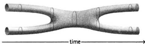
Figure 12.3 Strings interact by joining and splitting.
