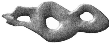
Figure 9.2 The shape of a multihanded doughnut can be deformed in many ways, one of which is illustrated here, without changing the number of holes it contains.
