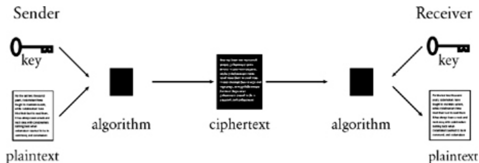
Figure 4 To encrypt a plaintext message, the sender passes it through an encryption algorithm. The algorithm is a general system for encryption, and needs to be
