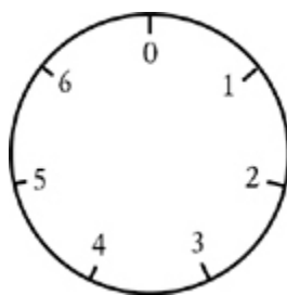
Figure 64 Modular arithmetic is performed on a finite set of numbers, which can be thought of as numbers on a clock face. In this case, we can work out 6 + 5 in modular 7 by starting at 6 and moving around five spaces, which brings us to 4.
