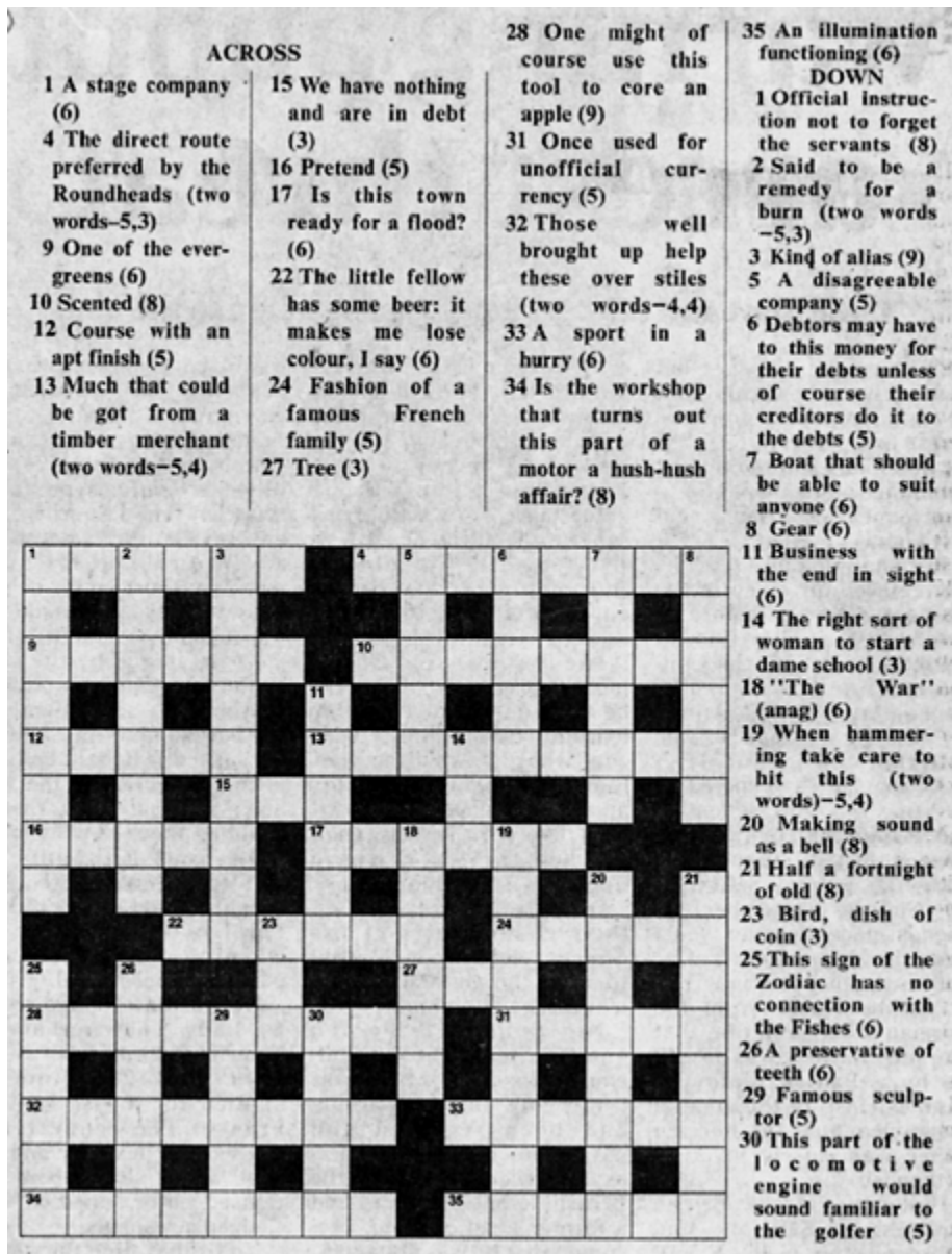
Figure 51 The Daily Telegraph crossword used as a test to recruit new codebreakers (the solution is in Appendix H ). (photo credit 4.6)
