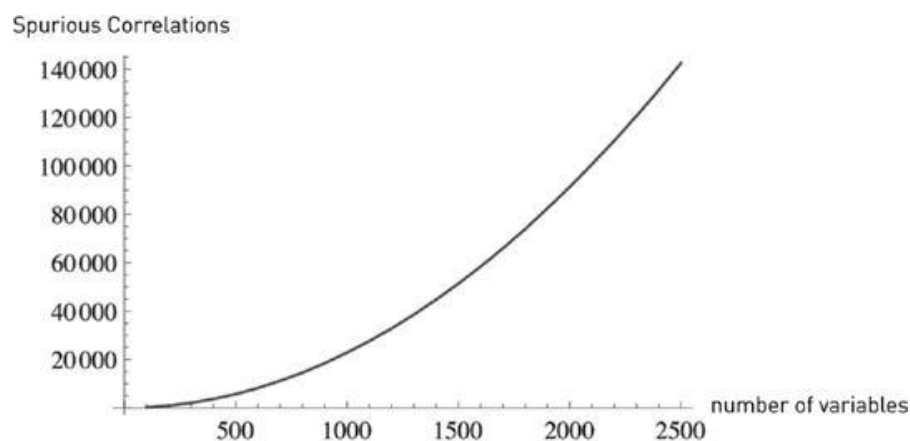
FIGURE 18. The Tragedy of Big Data. The more variables, the more correlations that can show significance in the hands of a “skilled” researcher. Falsity grows faster than information; it is nonlinear (convex) with respect to data.
