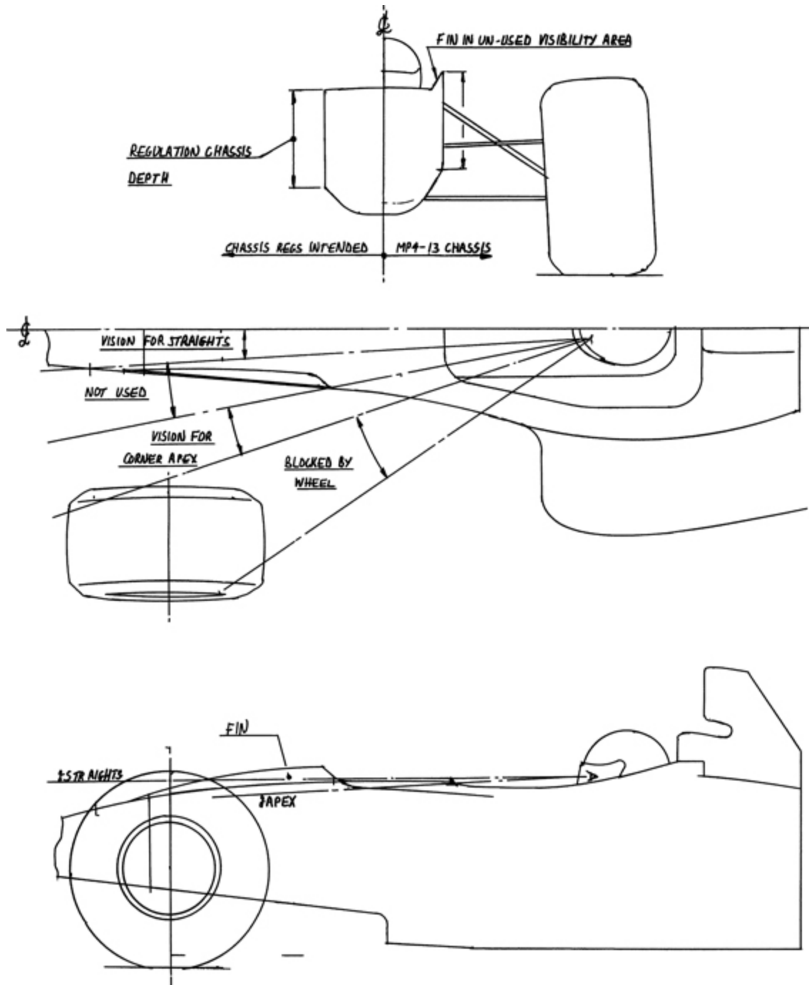
Figure 15: The consequences for the driver's vision of the depth-in-section regulation for the MP4 13.
