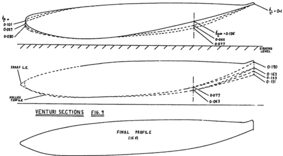
Figure 5: Technical drawing from my university project, illustrating 2D sections of the underside wing shape (venturi).
