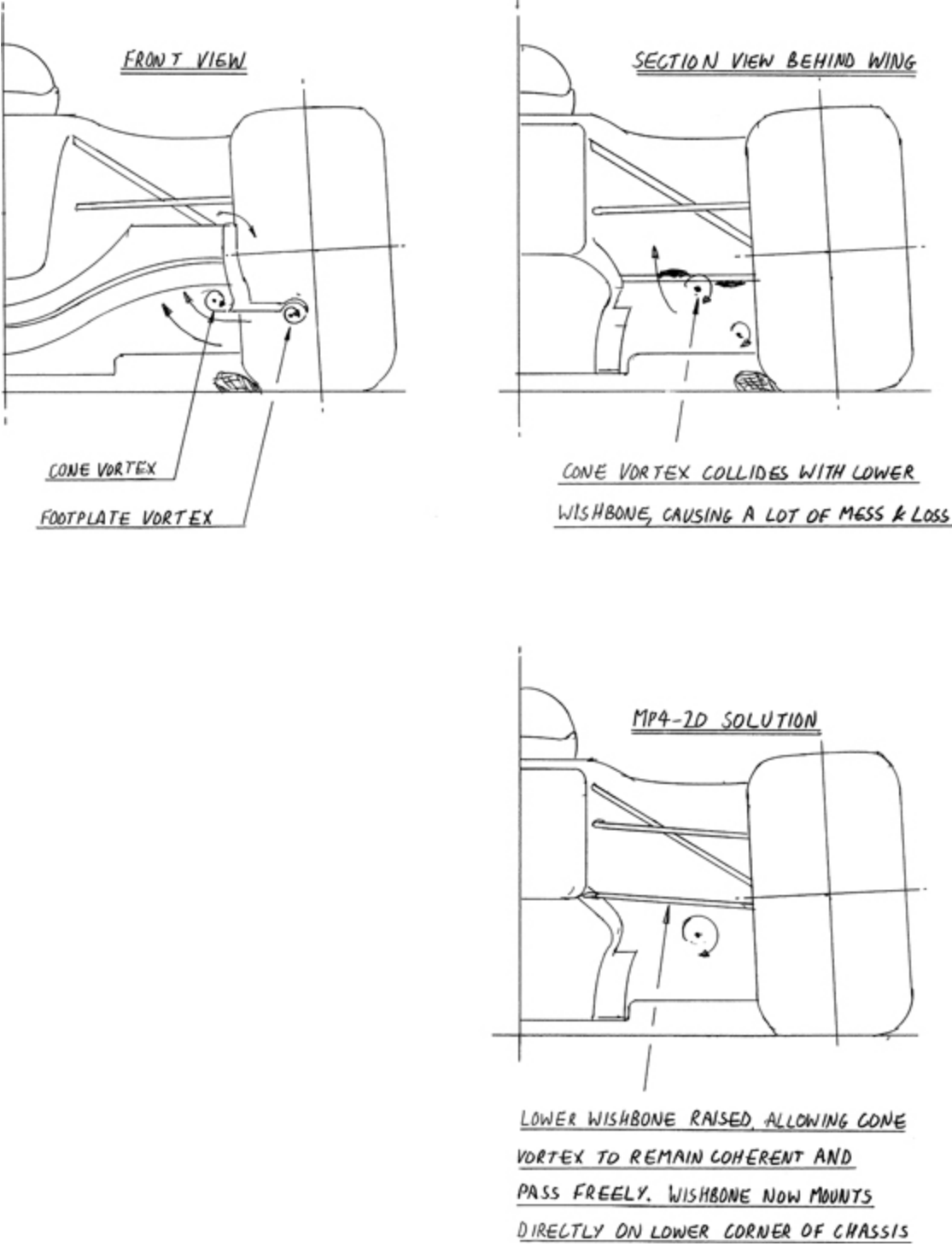
Figure 16: Our solution to the aerodynamic problems on the front wing of the MP4 20, which were caused by regulations requiring it to be raised by 50mm.
