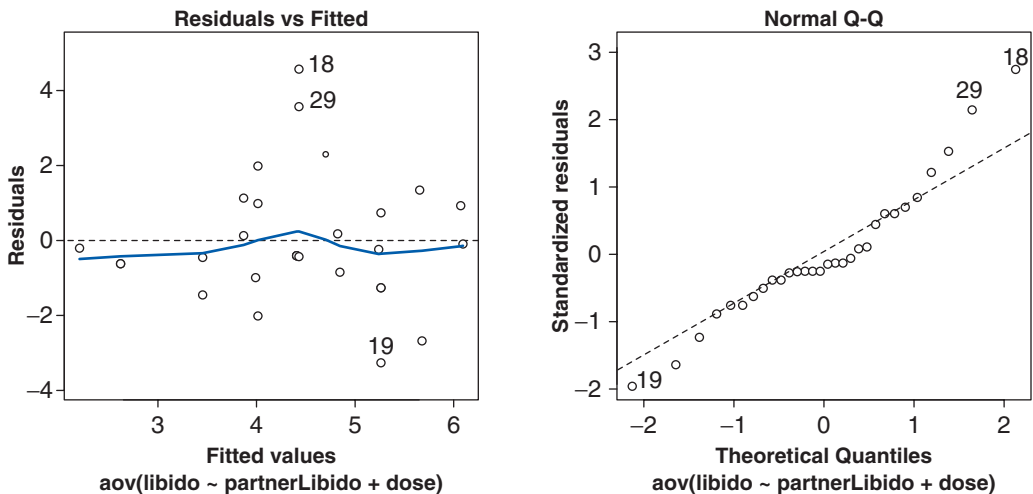
FIGURE 11.6 Plots of an ANCOVA model
