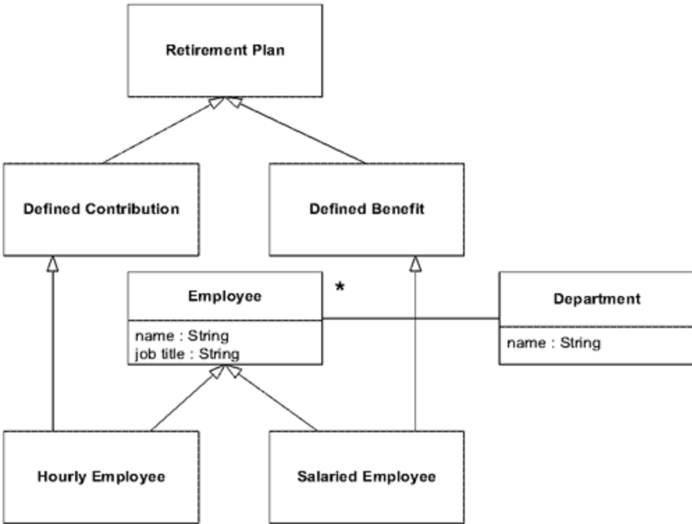
Figure 16.16. Some employees represented using the old model
