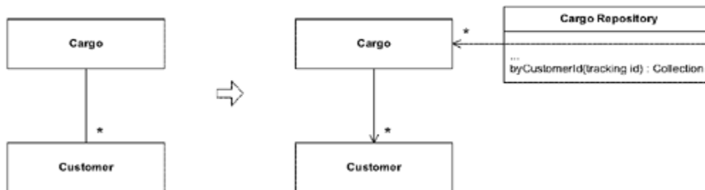
Figure 16.6. A first-pass layered model
