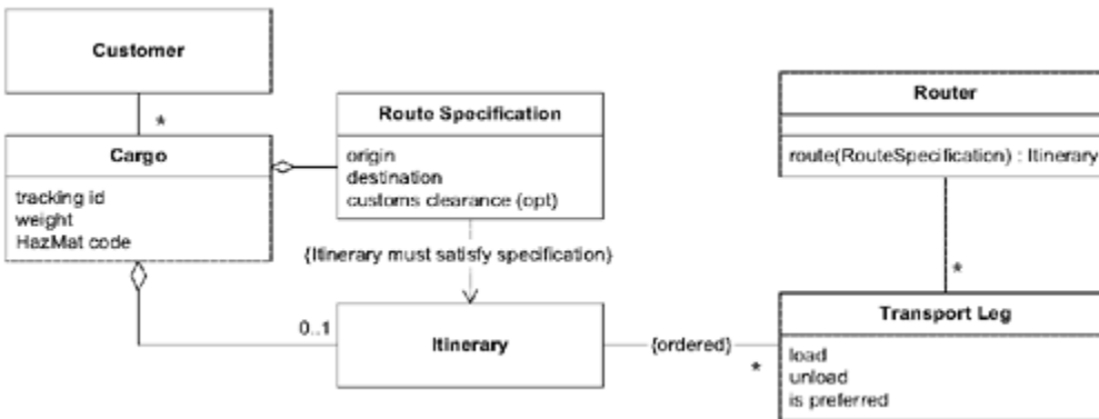
Figure 16.4. Using the model to route a cargo during booking
