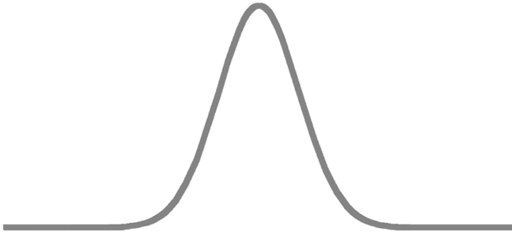
FIGURE 10: A MORE ABSTRACT VERSION: PLATO'S CURVE
