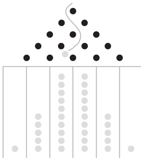
FIGURE 8: THE QUINCUNX (SIMPLIFIED)—A PINBALL MACHINE
