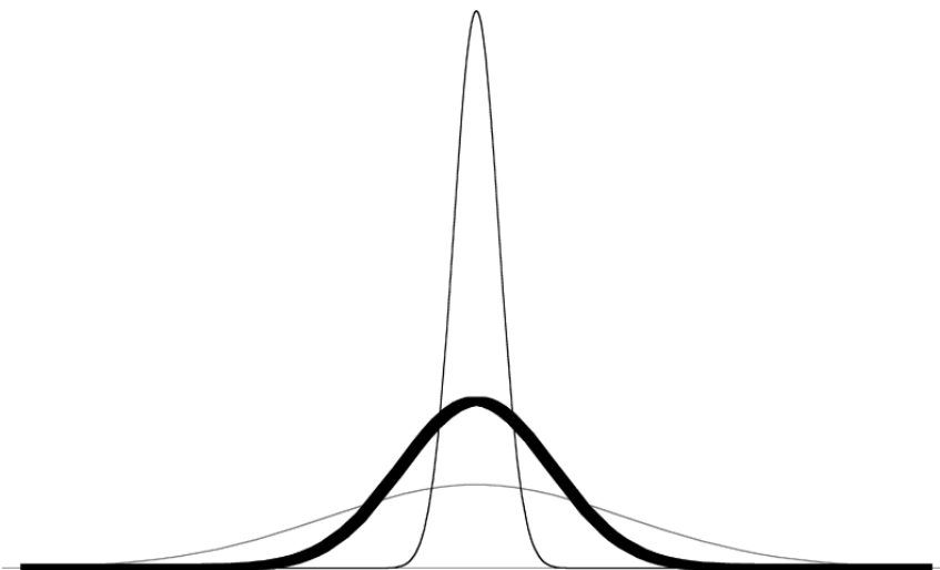
FIGURE 7: How the Law of Large Numbers Works
