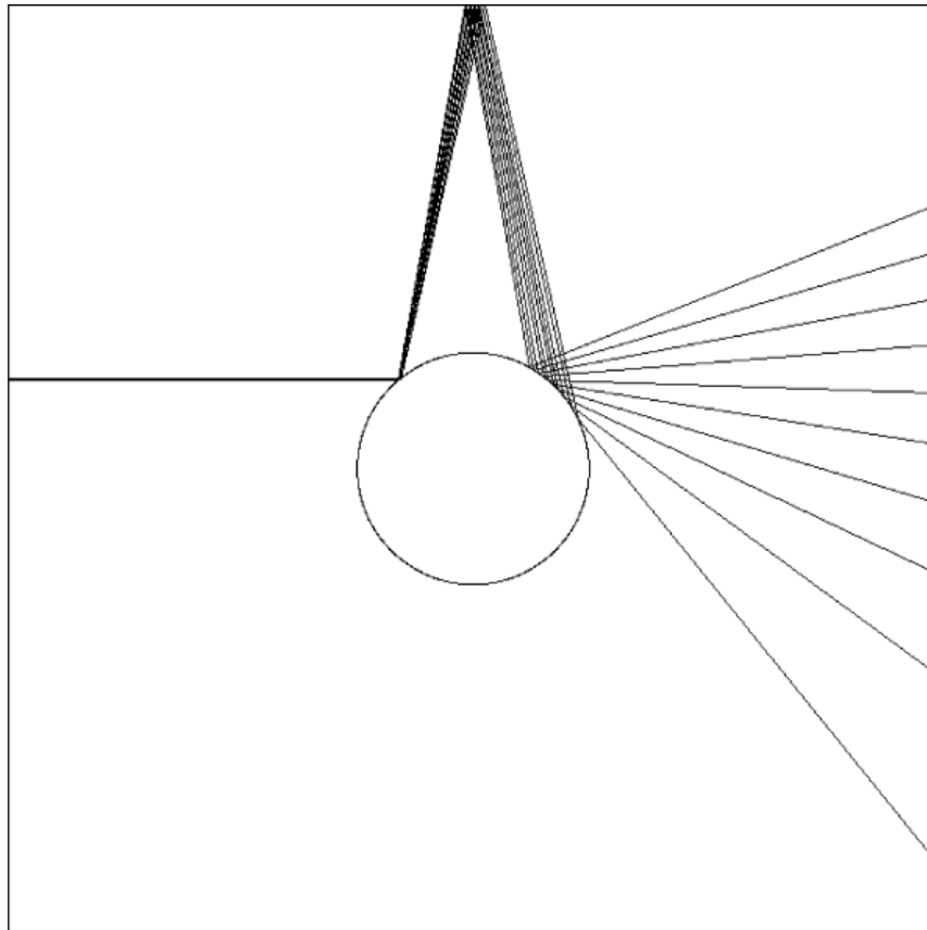
FIGURE 2: PRECISION AND FORECASTING
