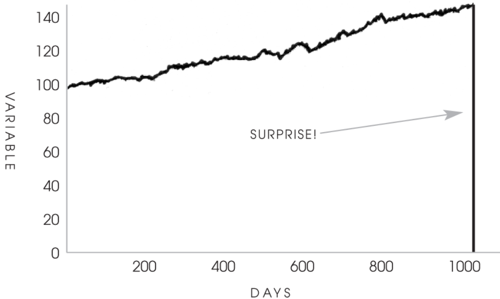
FIGURE 1: ONE THOUSAND AND ONE DAYS OF HISTORY
