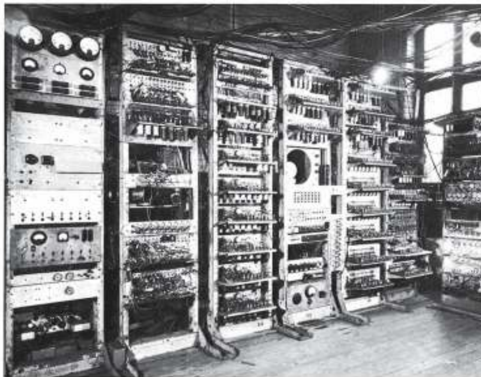
Above: The prototype Manchester computer. The six racks shown are essentially those of the 'baby machine' which ran its first program in June 1948; by June 1949 when this photograph was taken, the machine had roughly doubled in size.
